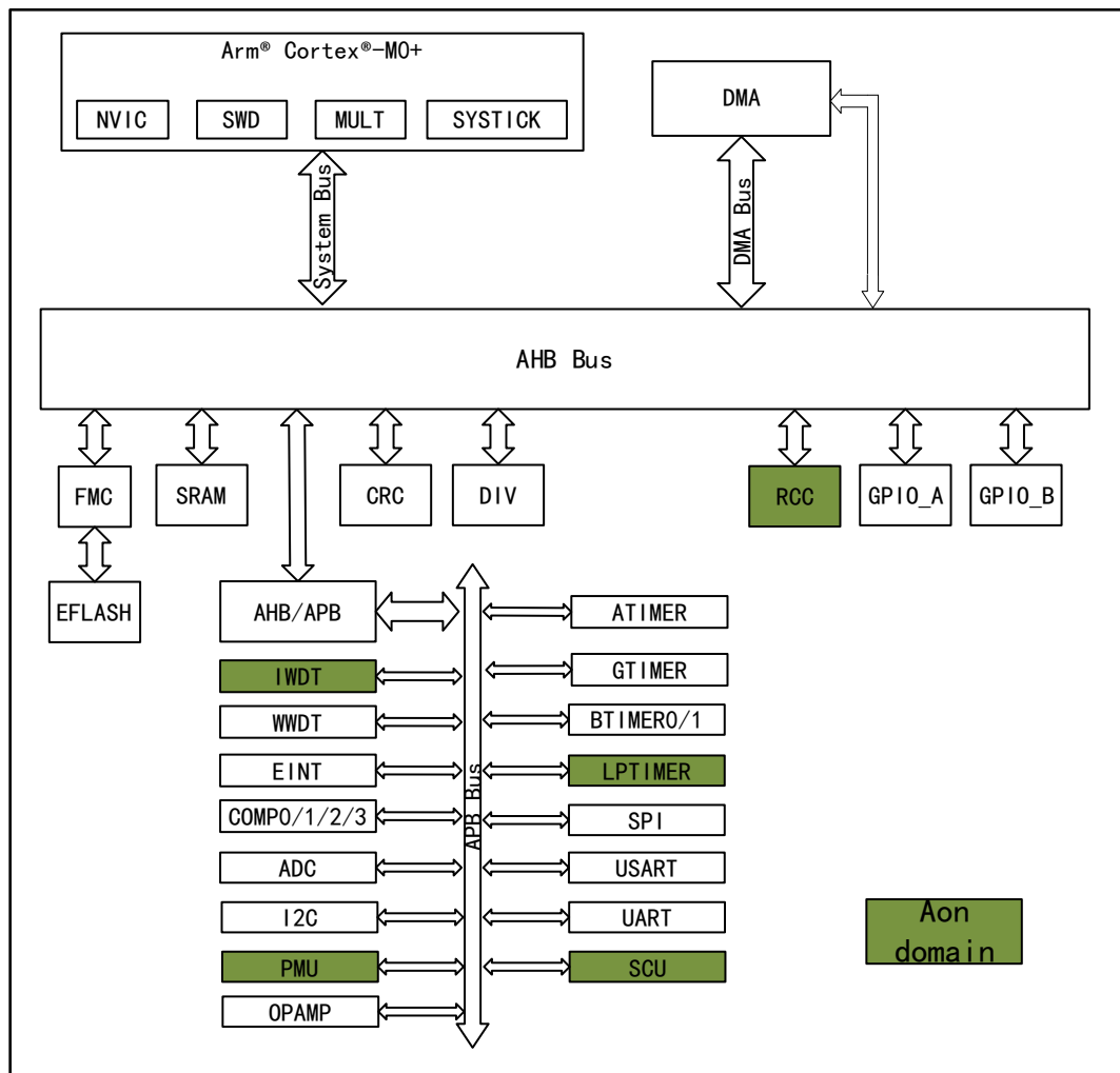
Figure 2 System Architecture Block Diagram
