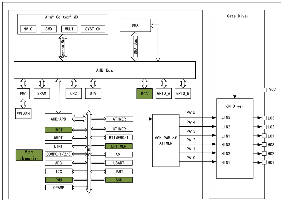
Figure 4 System Architecture Block Diagram
