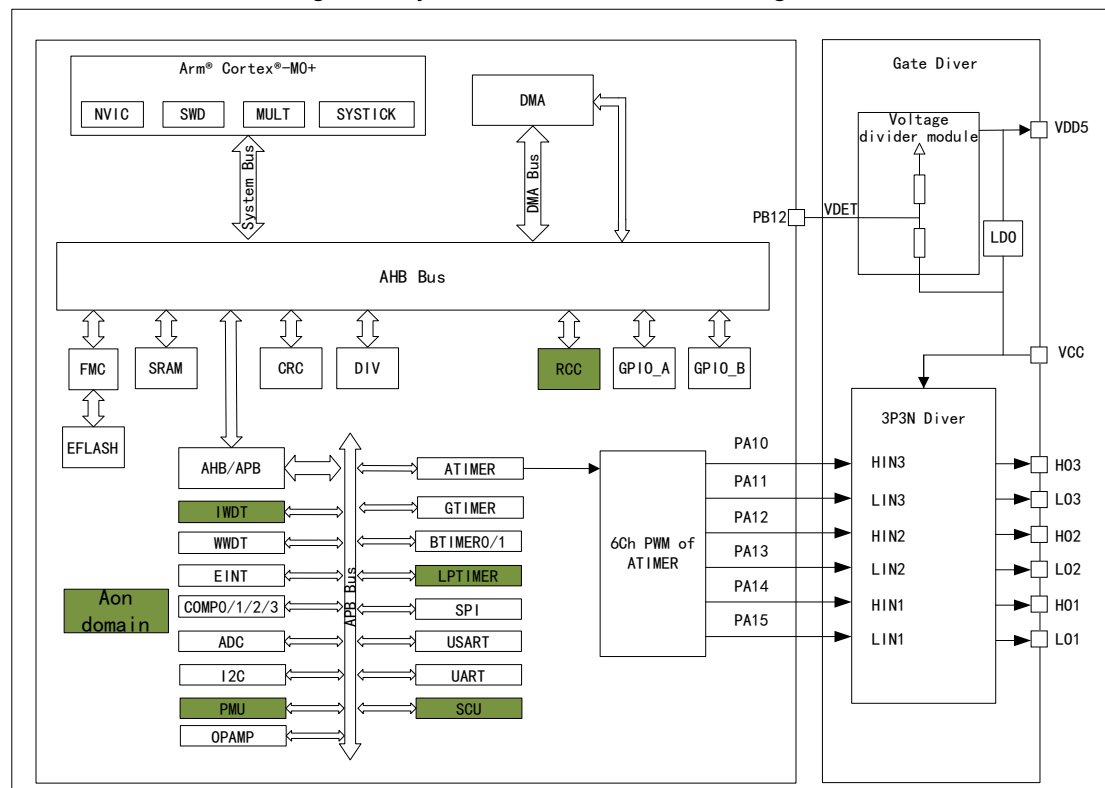
Figure 5 System Architecture Block Diagram
