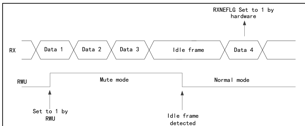
Figure 73 Idle Bus Exit Mute Mode
