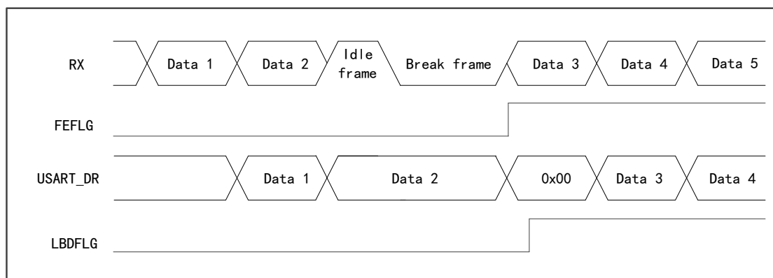
Figure 79 Break Frame Detection in Idle State
