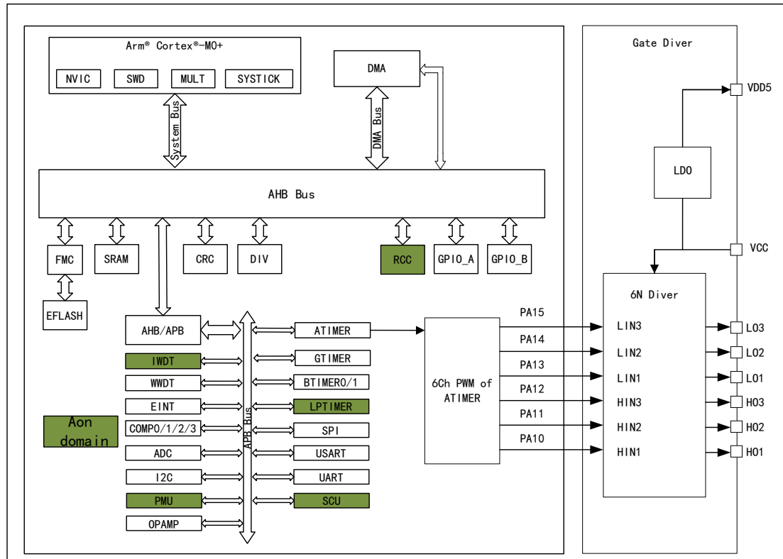
Figure 3 System Architecture Block Diagram
