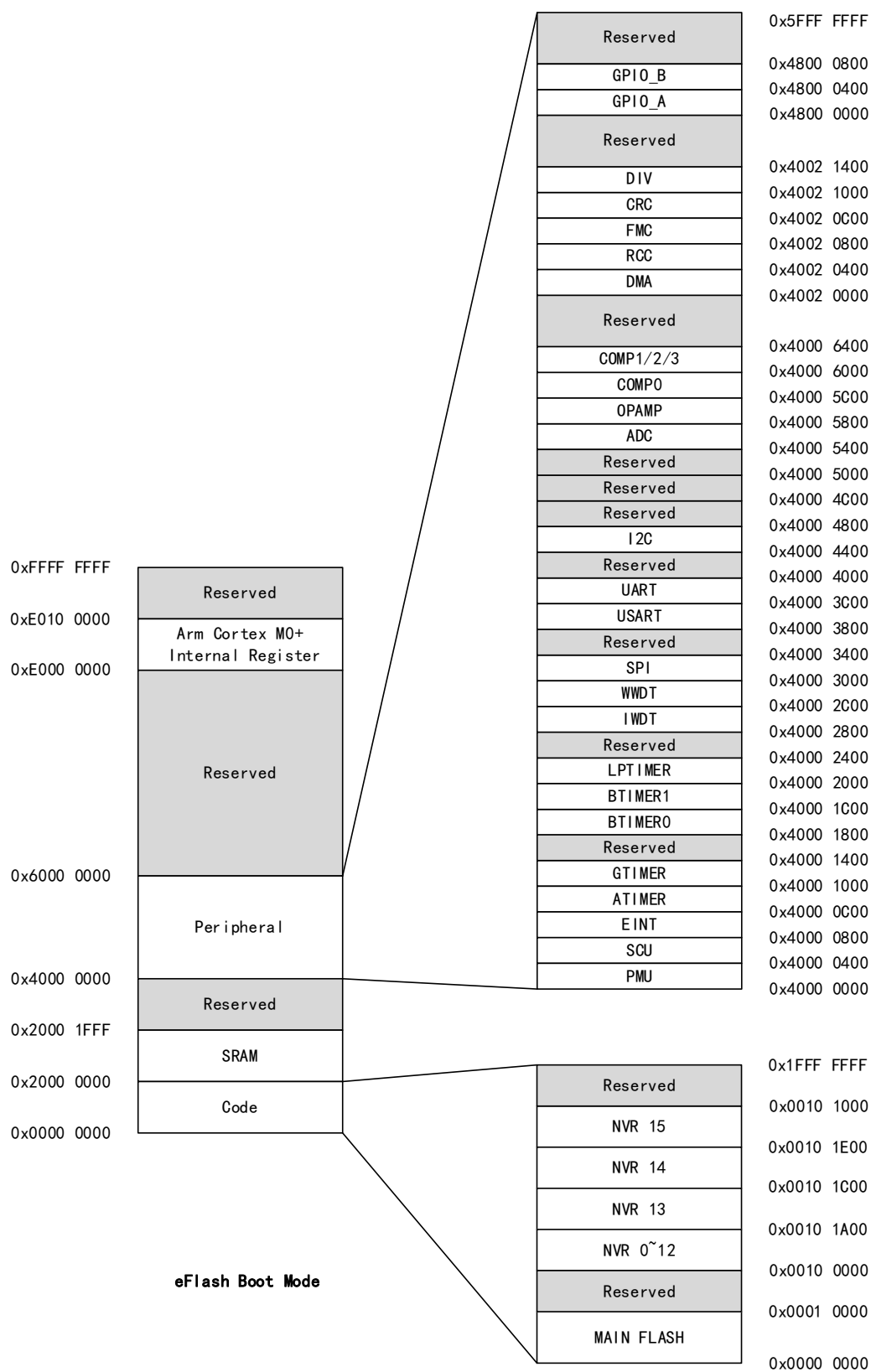
Figure 6 Address Mapping
