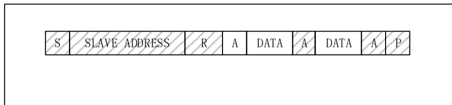
Figure86 Master Reads Data from Slave
