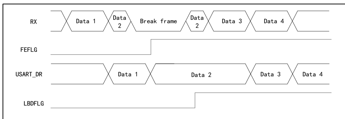
Figure 80 Break Frame Detection in Data Transmission State
