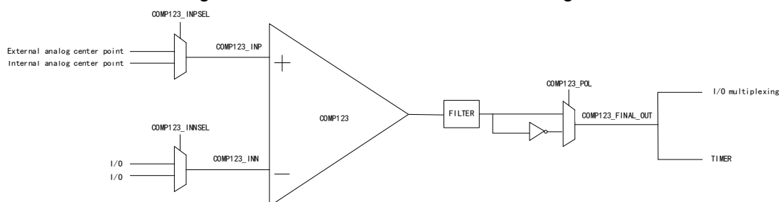
Figure 108 COMP1/2/3 Structure Block Diagram
