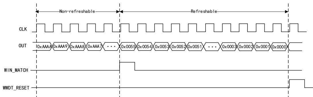
Figure 70 Timing Diagram
